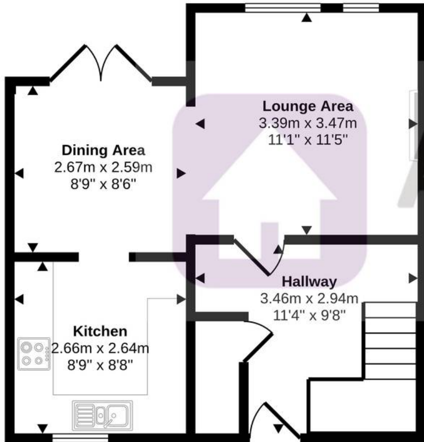
Ground Floor Approx 38 sq m / 404 sq ft
